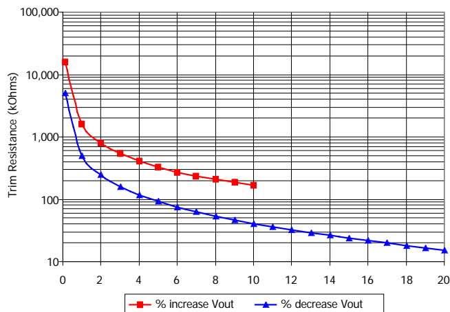
Figure C: Trim Graph for 5.0 Vout module
